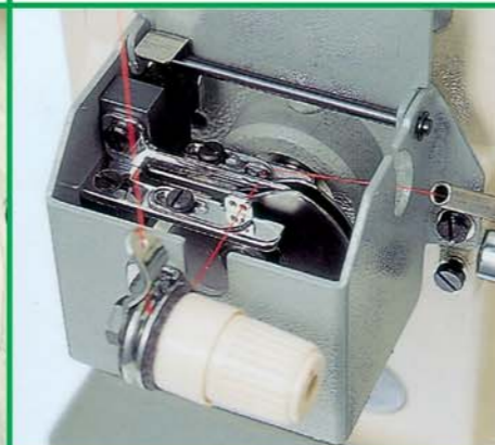
采用下饰打线器结构及过线引导改良。 Featuring lower ornament thread feeding and modified excess guides.
