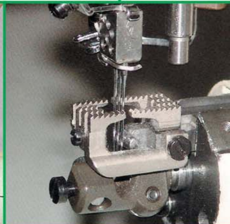
采用调节式主输送齿及活动针挡。 Regulating main feeding gear and movable needle guard.
